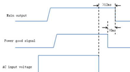
Figure 19. Power good signal sequence
