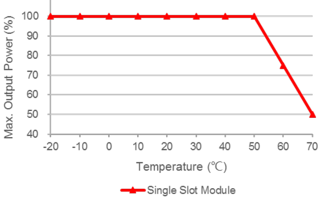
Max. Output Power Derating Curves
