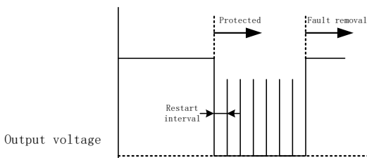
Figure 16. Auto-Recovery
